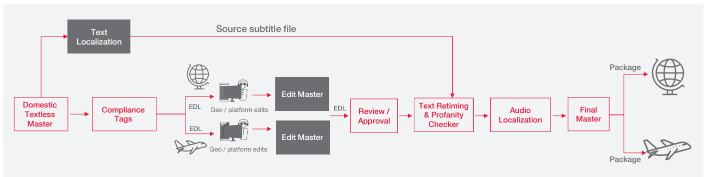
Workflow for Global Versioning on CLEAR Media ERP
